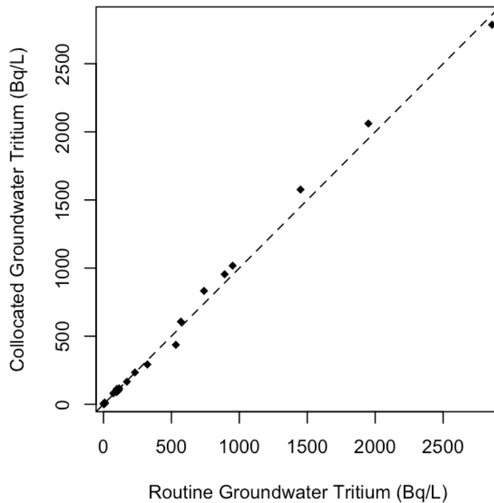
Figure 8-1. Example of good agreement between collocated sample results using groundwater tritium concentrations.
